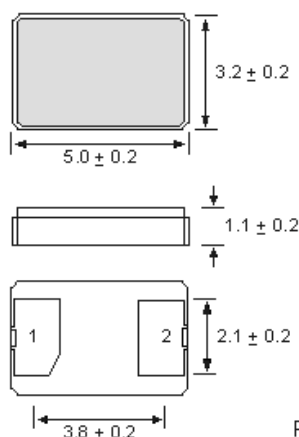
Internal Connections Top view
