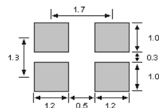
Recommended Soldering Pattern
